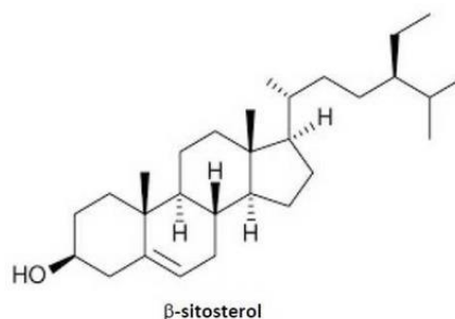
\beta -sitosterol
